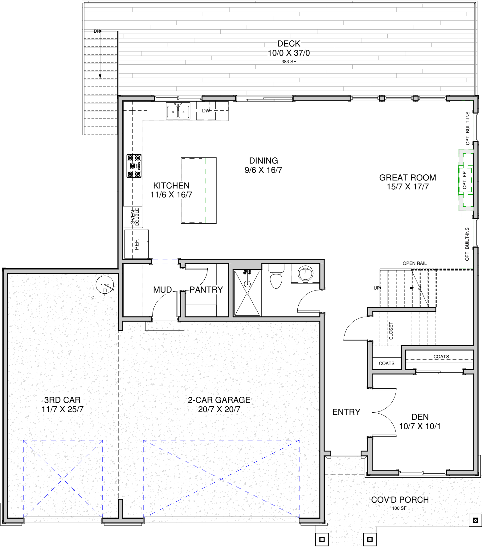
MAIN FLOOR - 1,127 SF
