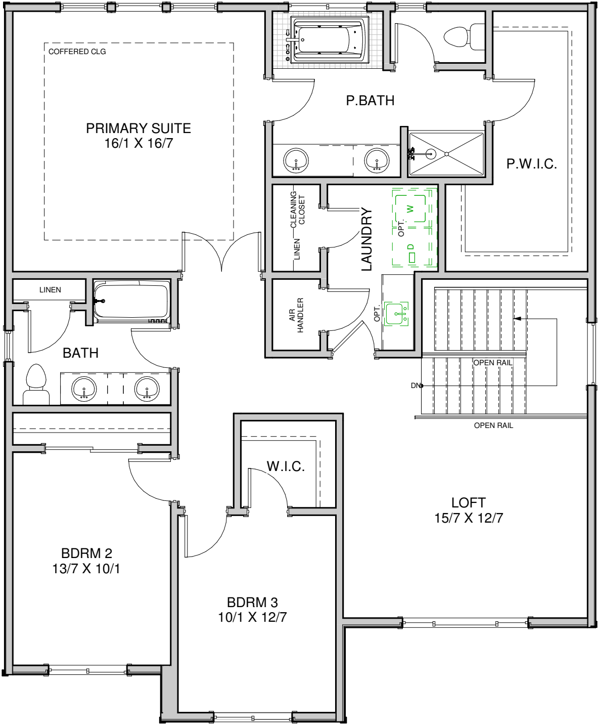
UPPER FLOOR - 1,492 SF
