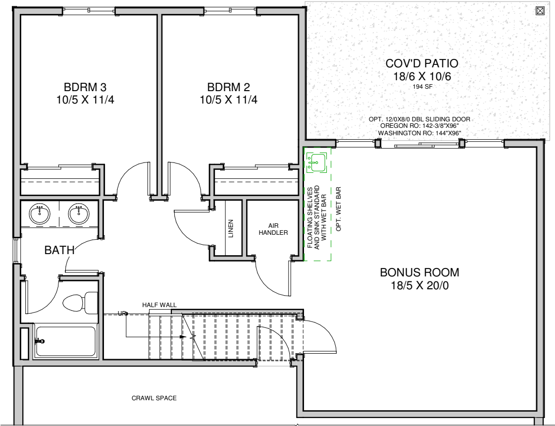
LOWER FLOOR - 973 SF
