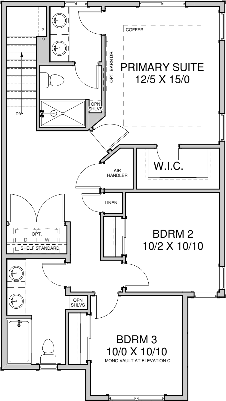
UPPER FLOOR - 908 SF
