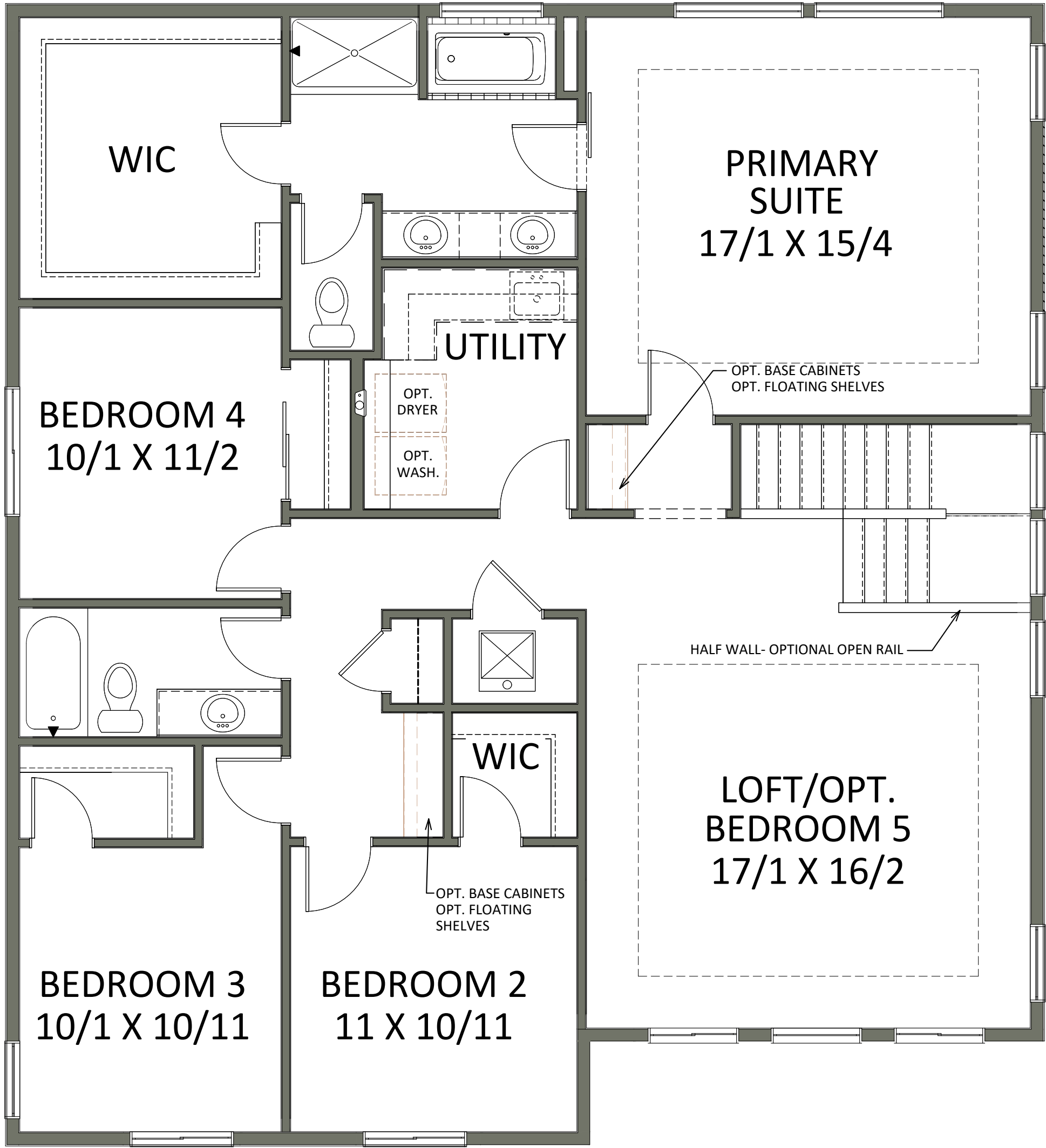
UPPER FLOOR - 1624 SF
