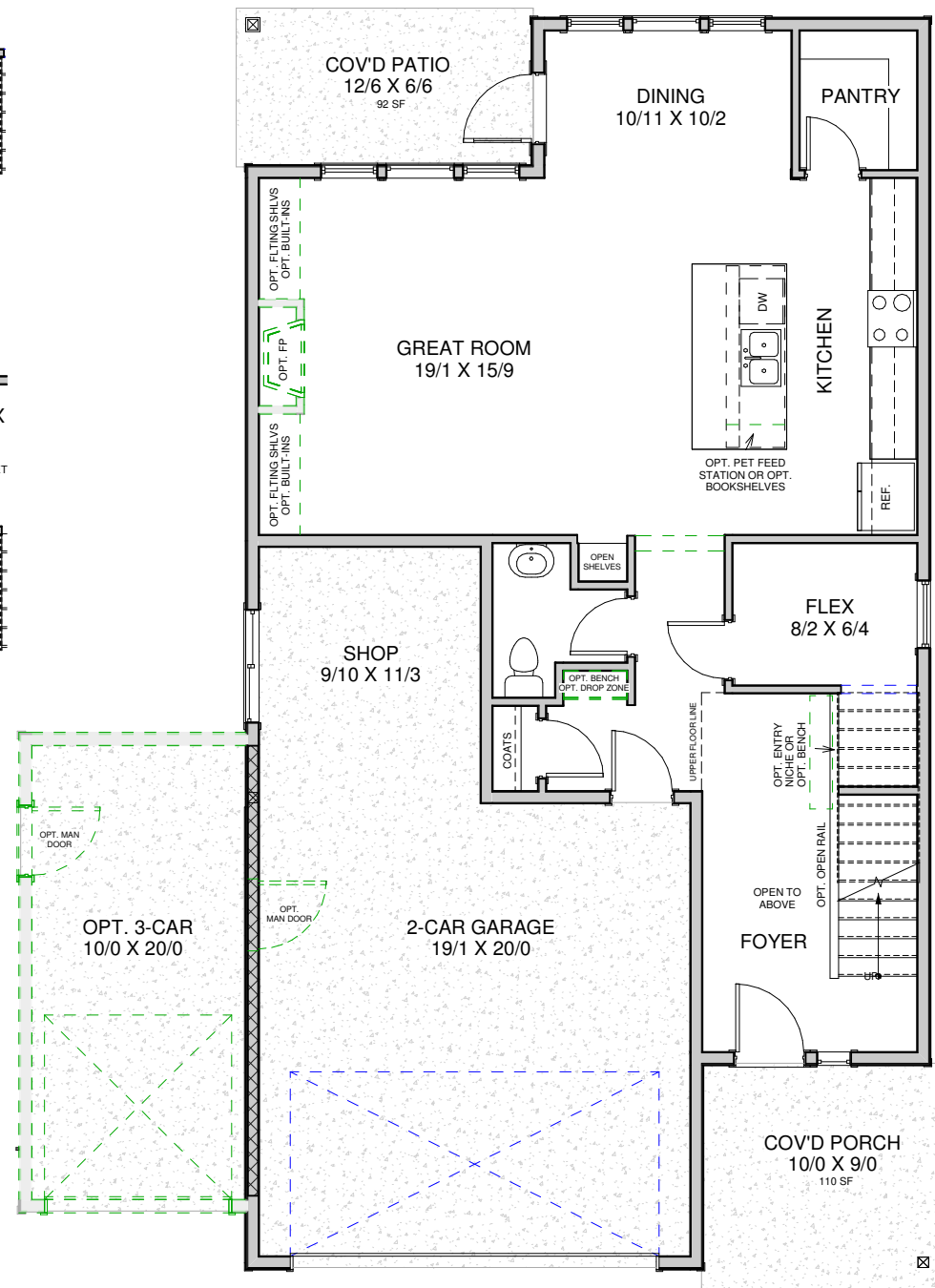
MAIN FLOOR - 957 SF
