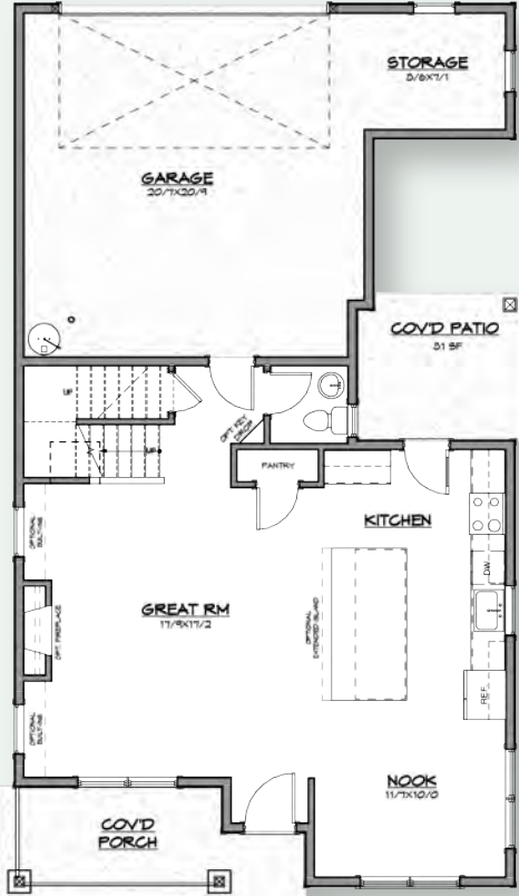
MAIN LEVEL
