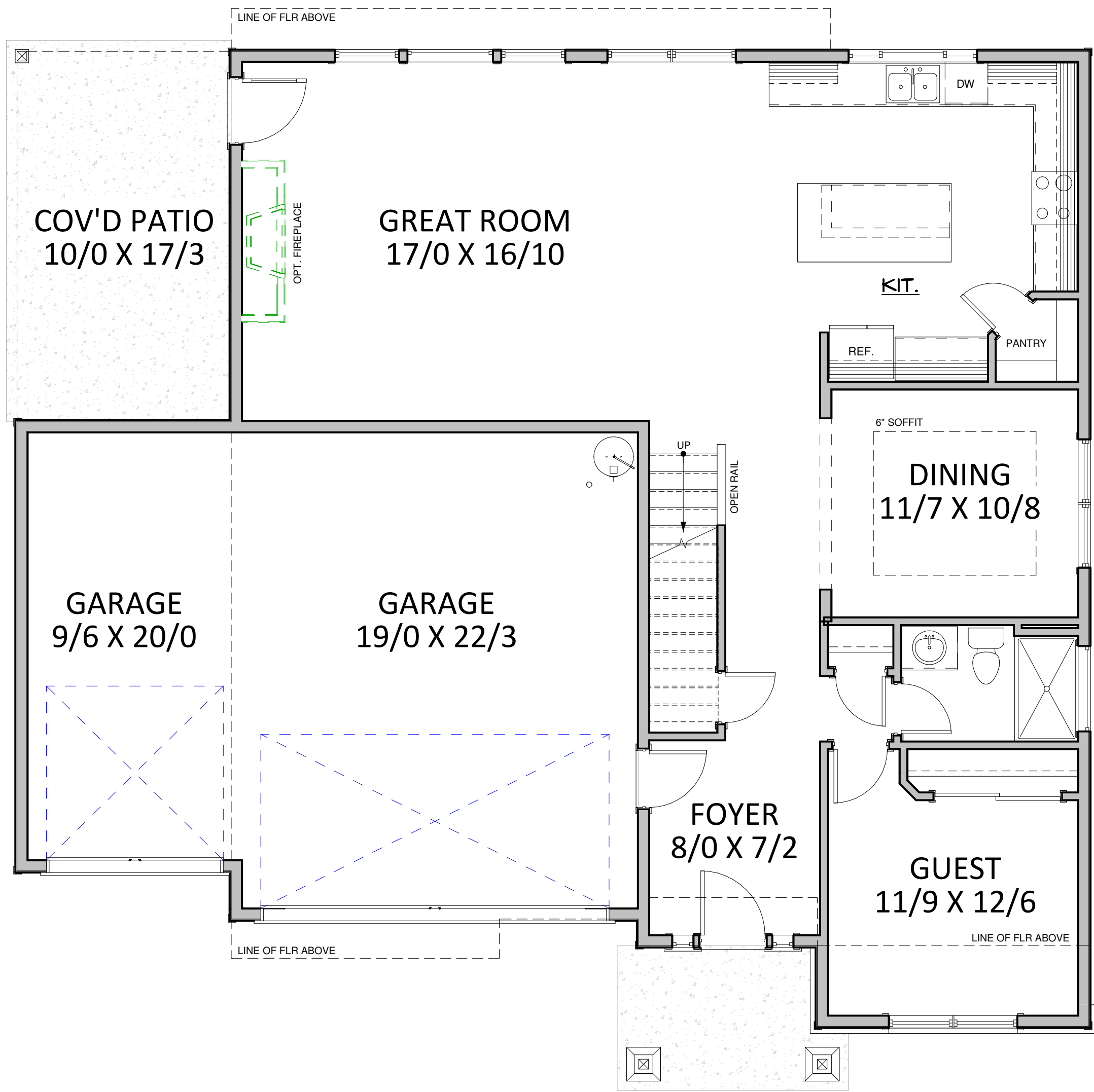
MAIN FLOOR - 1261 SF
