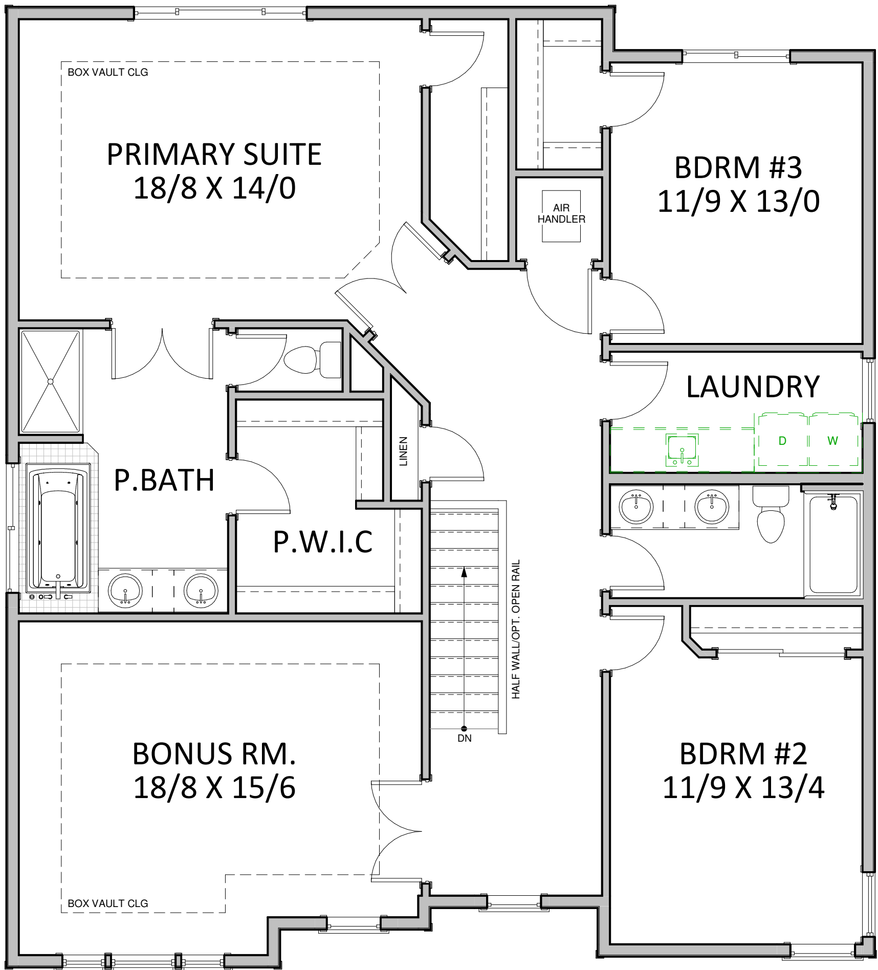
UPPER FLOOR - 1667 SF
